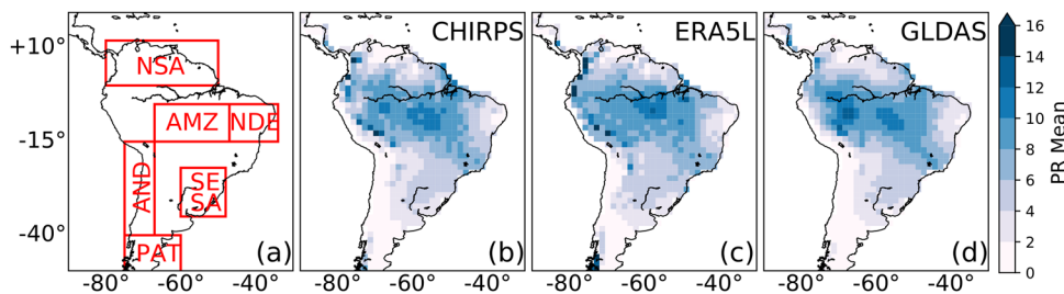
FIGURE 1 (a) The six regions of SA analysed in the study; (b–d) NDJFM mean PR ( \text{mm}\cdot\text{day}^{-1} ) from (b) CHIRPS (observed), (c) ERA5L (reanalysis) and (d) GLDAS (reanalysis) over 1999–2010
