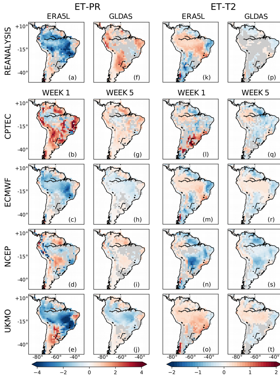
FIGURE 7 Same as Figure 6 but (a–j) for A_{CI} between ET and PR (mm·day -1 ) and (k–t) for A_{CI} between ET and T2 (K)
